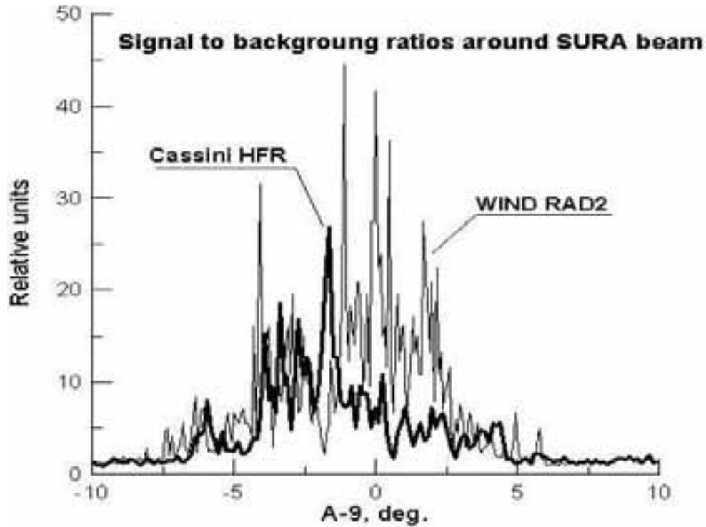
Figure 3: Signal-to-background ratios at 9025 kHz for the HFR u -monopole (boldface line) and the RAD2 Z -antenna (lightface line) in the case where the WIND and Cassini spacecraft are normalized to the same distance and to the same receiver's bandwidth (see text). Abscissa is the azimuthal difference \delta A = A - 9^\circ relative to the SURA emission peak.
