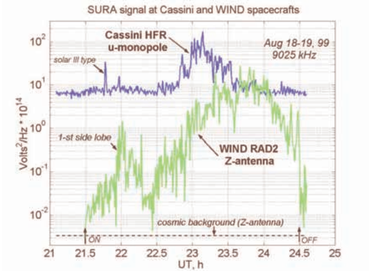
Figure 2: Measured signals onboard the Cassini and WIND spacecraft with log-scale for signal power in units V^2/Hz at 9025 kHz. Dashed lines show cosmic background level for HFR u -monopole and RAD2 Z-antenna. Arrows (marked ON and OFF) denote the times when SURA was switched on and off. A solar type III event near 21:47 UT is also indicated.
