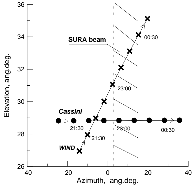
Figure 1: Sky positions of the Cassini and WIND spacecraft around the SURA beam in Aug 18–19, 1999. The spacecraft trajectories are indicated by solid lines with bold circles and crosses respectively, numbers near the marks denote universal time. The hatched region is the projection of the SURA beam on the sky; dashed lines correspond to first zeros of antenna pattern.
