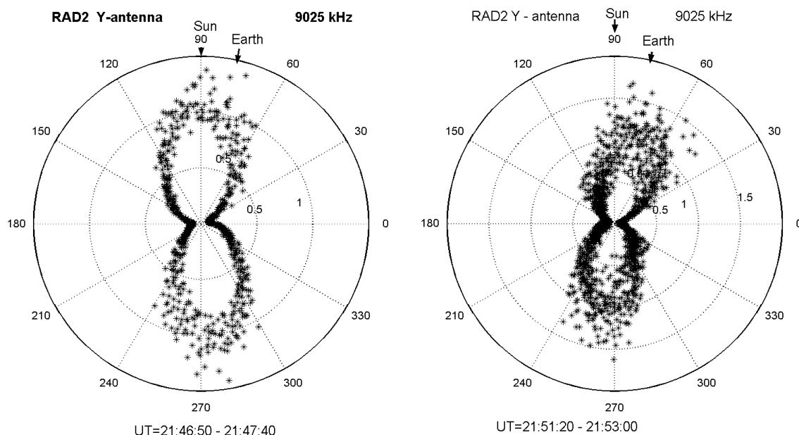
Figure 4: Polar angular diagrams of RAD2 Y-antenna response for solar type III burst (left panel) and for SURA side lobe emission (right panel). Azimuth A = 0 corresponds orientation of Y-antenna axis to the sun. Arrows indicate expected emission peaks for sun and ground-based sources in case of short antenna response.
