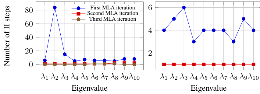
FIG. 5.5. Total number of steps required by the inverse iteration (II) at each individual iteration of MLA when computing the ten algebraically smallest eigenvalues of the matrices “nos3”. The initial eigenvalue approximation \sigma_0 for each sought eigenvalue \lambda was set to \sigma_0 = \lambda(1 + 1e-2) (left) and \sigma_0 = \lambda(1 + 1e-3) (right).
