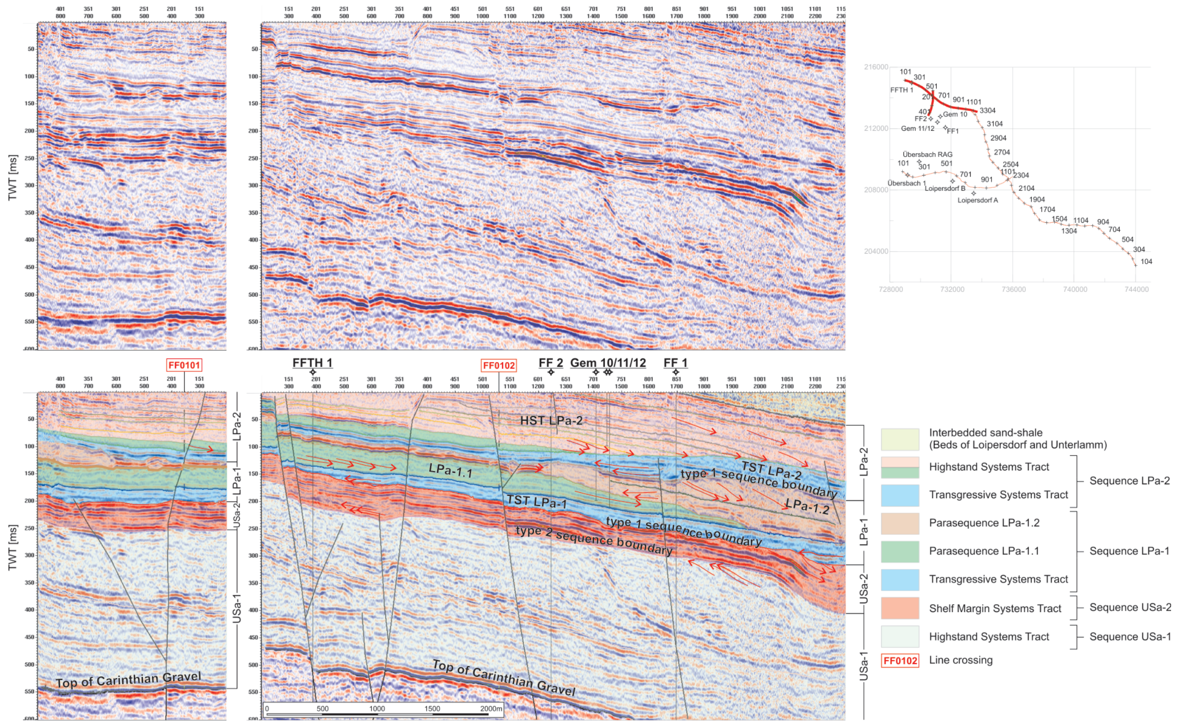
Fig. 3: Seismic line FF0101 and cross-line FF0102 and their interpretation. TWT – Two way travel time.
