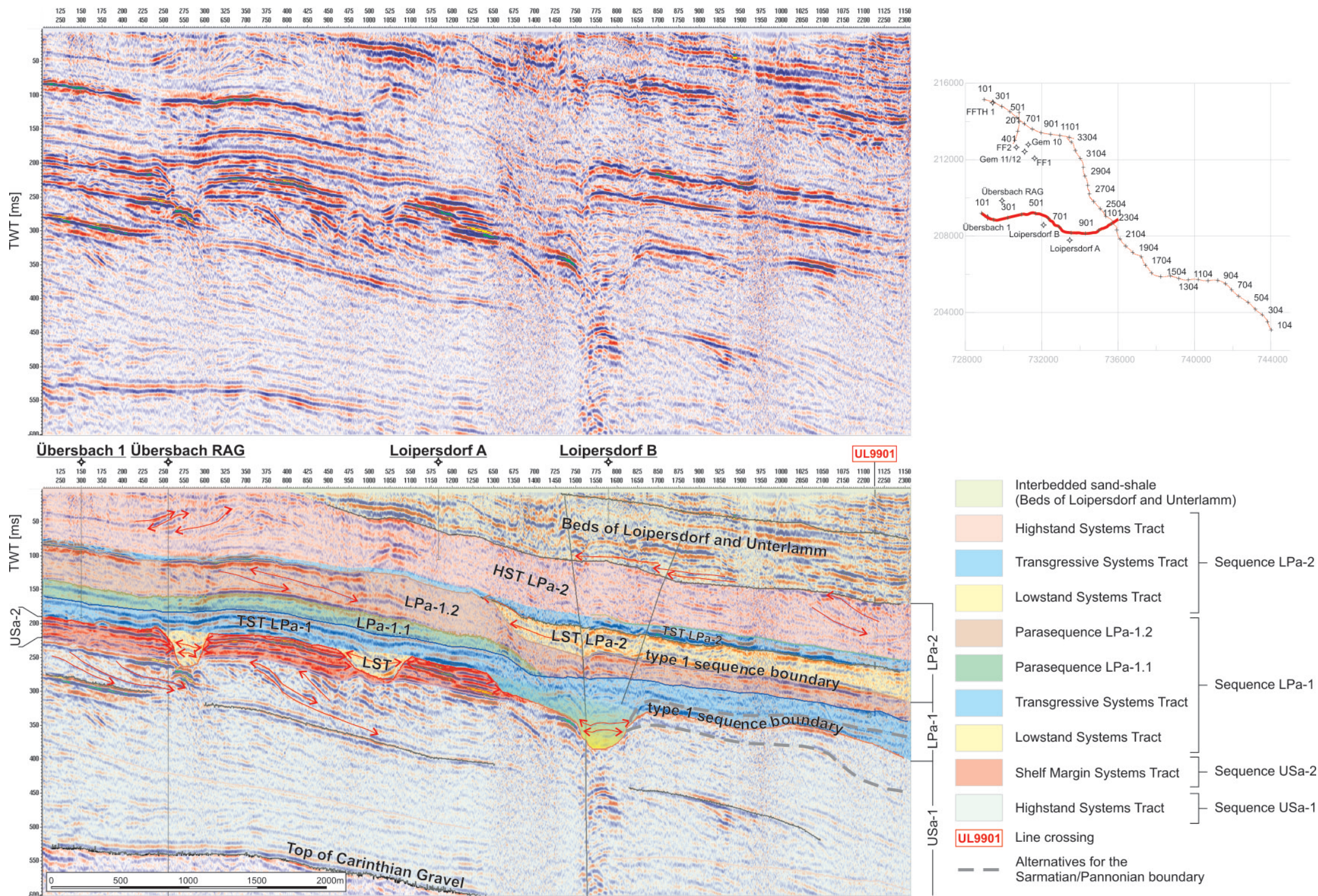
Fig. 5: Seismic line RI9901 and its interpretation. TWT – Two way travel time.
