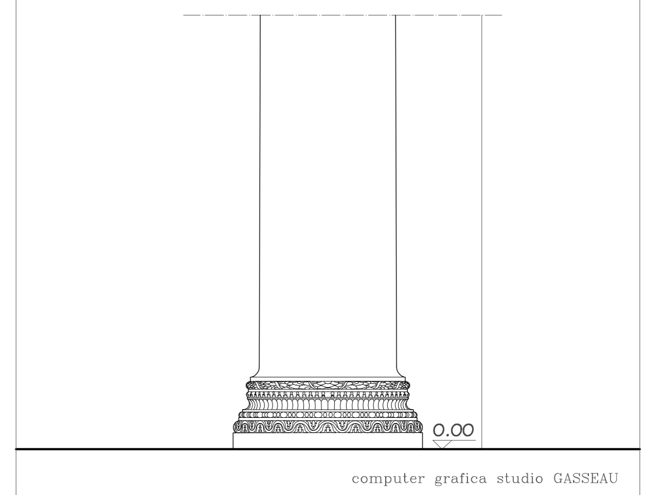
CARACALLATHERMEN – 'PALAESTRA' Detail 3 – 1:25
