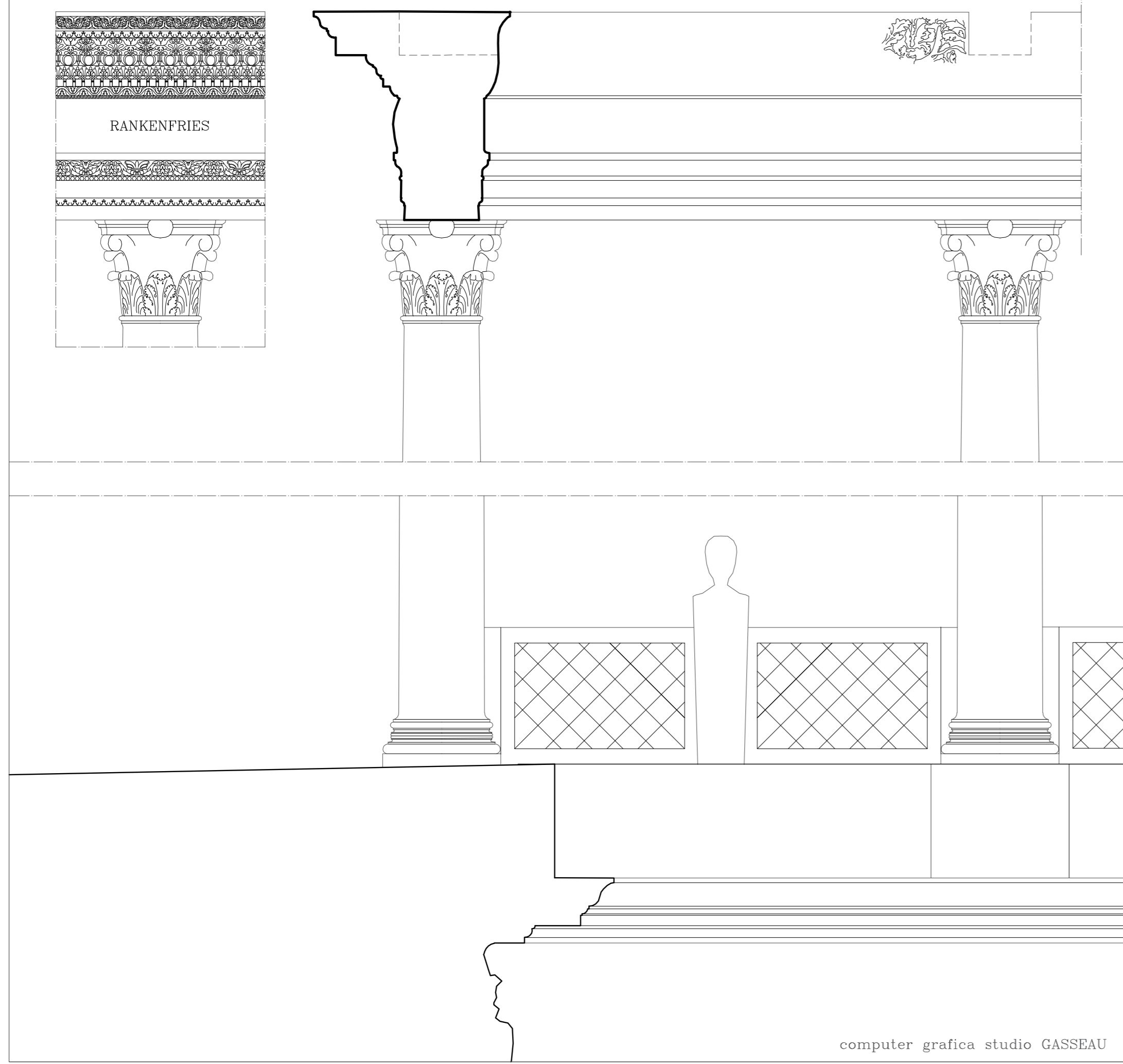
CARACALLATHERMEN – 'PALAESTRA' Detail 1 – 1:25
