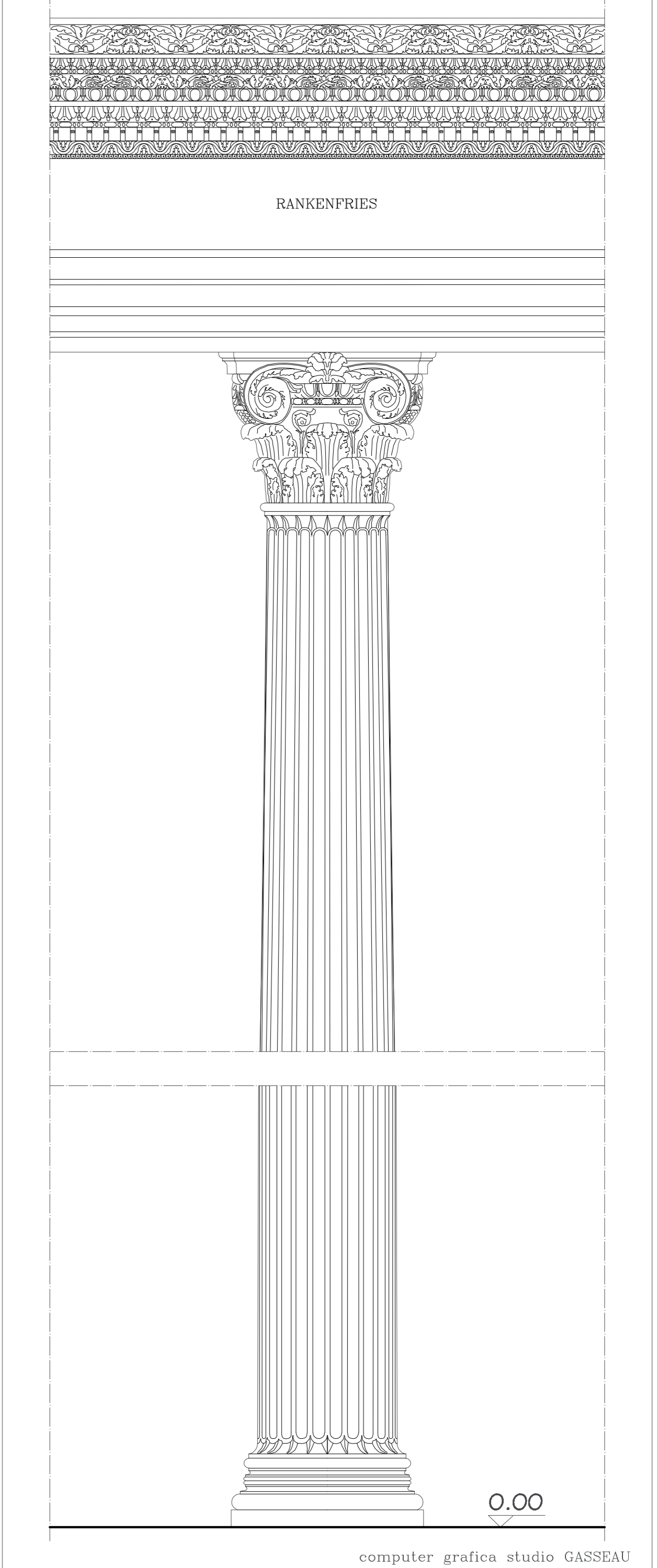
CARACALLATHERMEN – 'PALAESTRA' Detail 4 – 1:25
