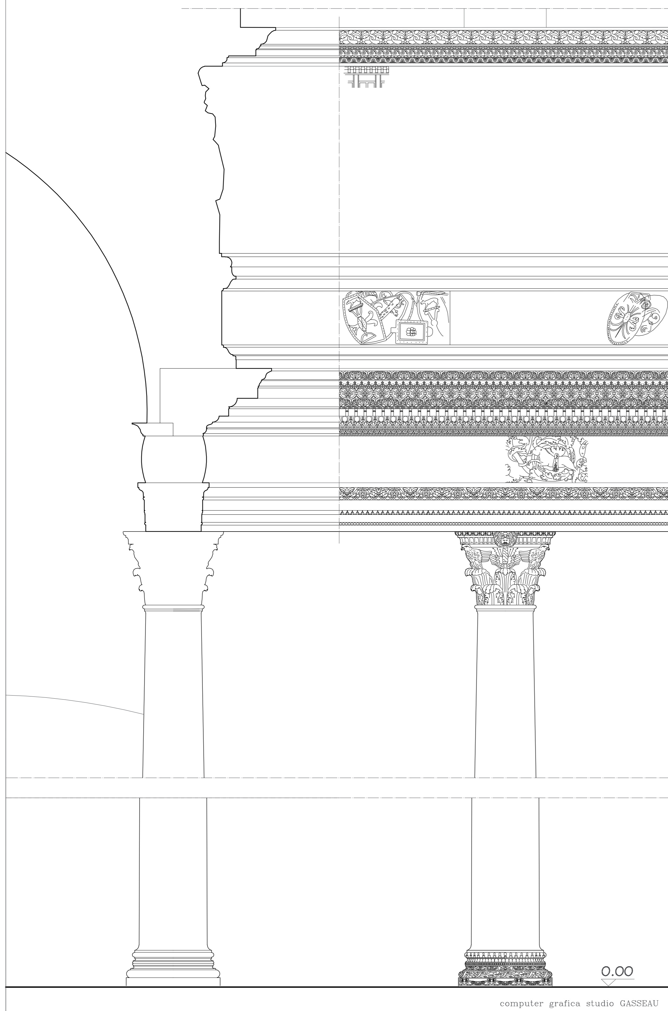
CARACALLATHERMEN – 'PALAESTRA' Detail 2 – 1:25
