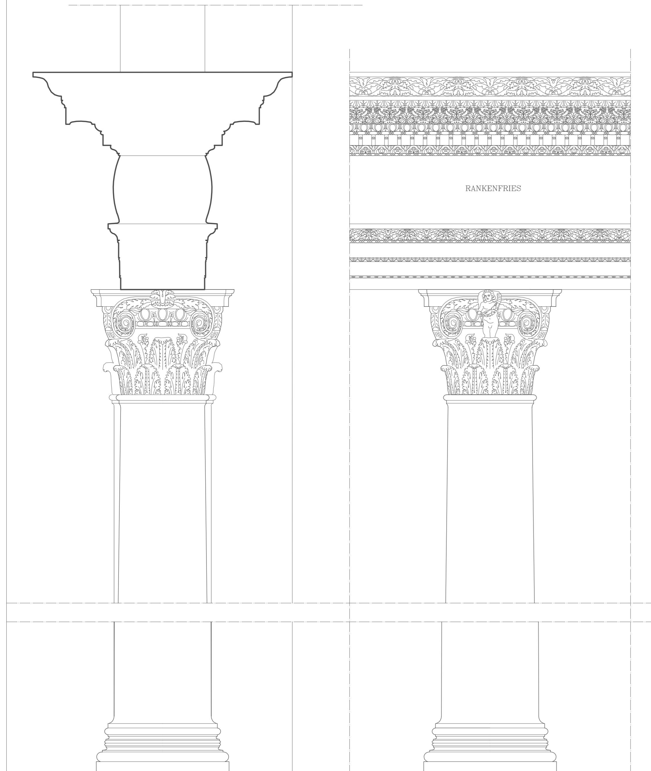
CARACALLATHERMEN – FRIGIDARIUM Detail 6a – 1:25
