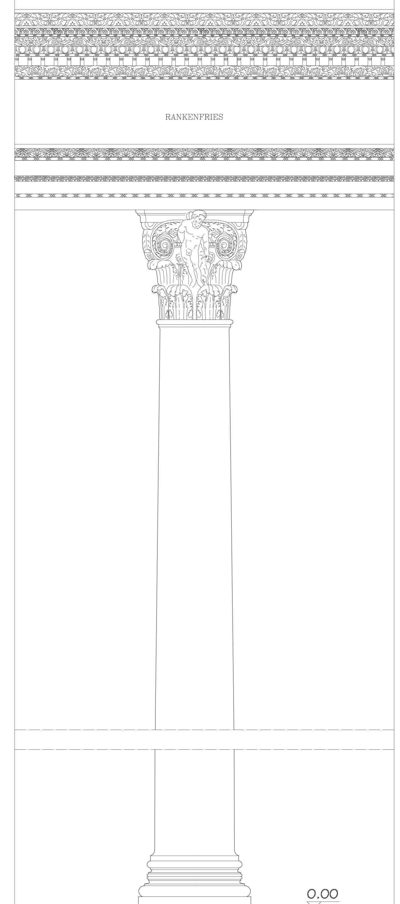
CARACALLATHERMEN – FRIGIDARIUM Detail 5 – 1:25
