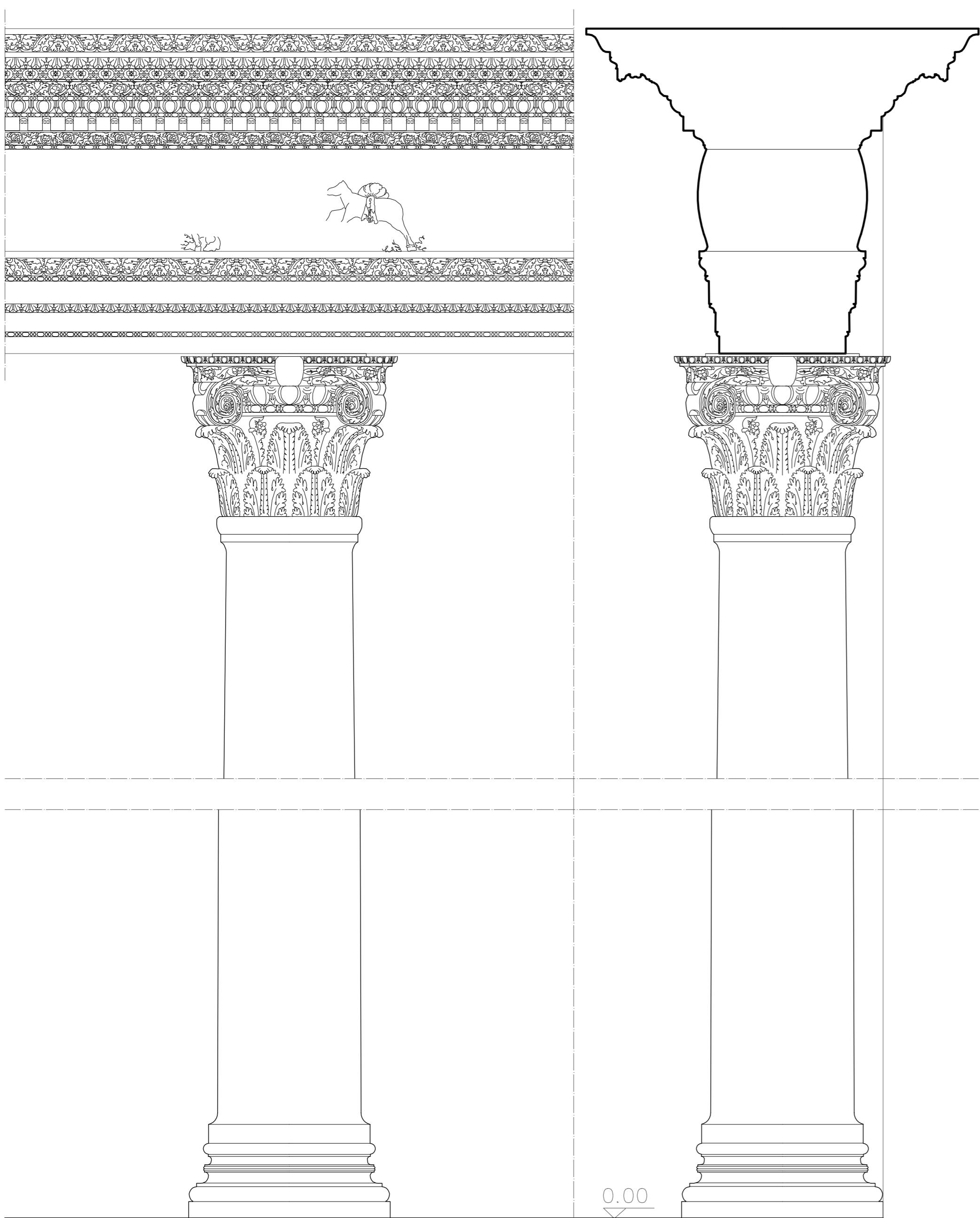
CARACALLATHERMEN – NATATIO Detail 7a – 1:25
