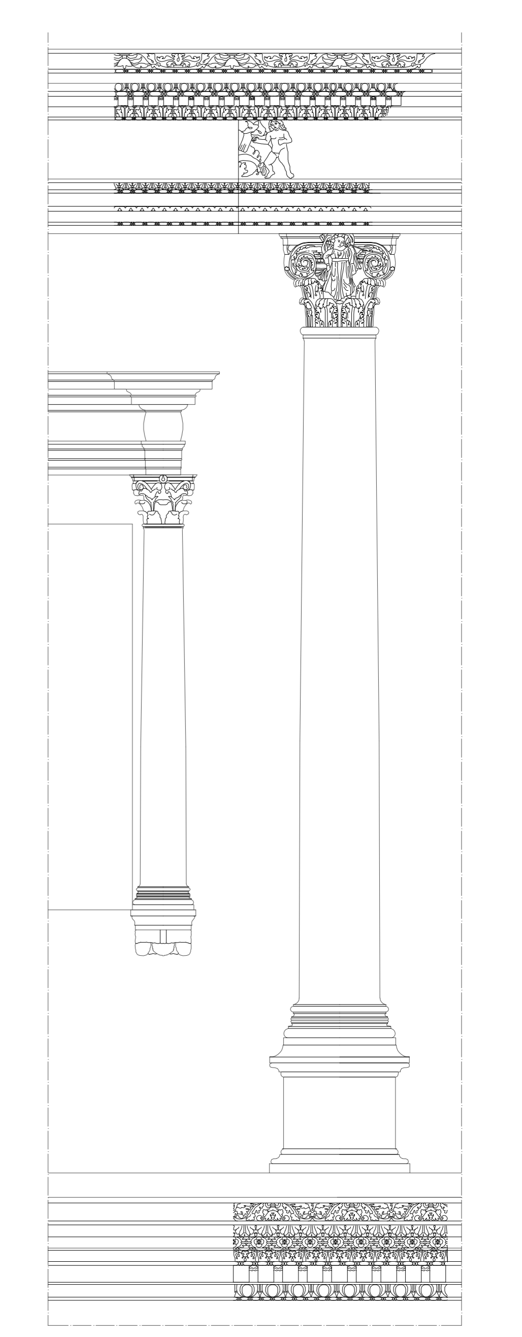
CARACALLATHERMEN – NATATIO Detail 10 – 1:25
