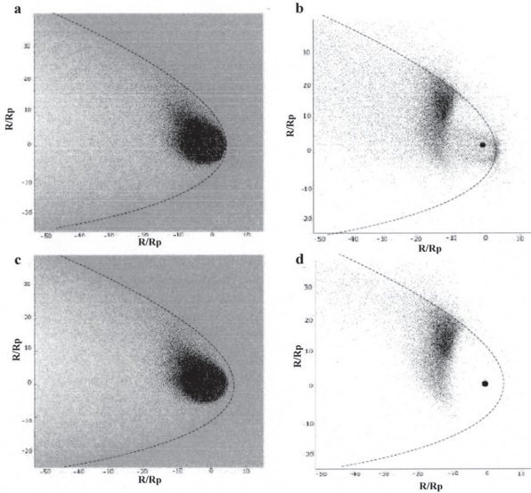
Figure 1: (a) Modelled stellar wind protons (bright gray area/dots), planetary and hydrogen ENAs (dark dots) around HD 209458b with an assumed sub-stellar magnetopause obstacle at 4.3R_p . (b) Only hydrogen atoms with velocities > 50 \text{ km s}^{-1} around HD 209458b for the same stellar wind parameters and planetary obstacle. (c) and (d) correspond to similar model runs but with a magnetopause stand-off distance at 6.3R_p .
