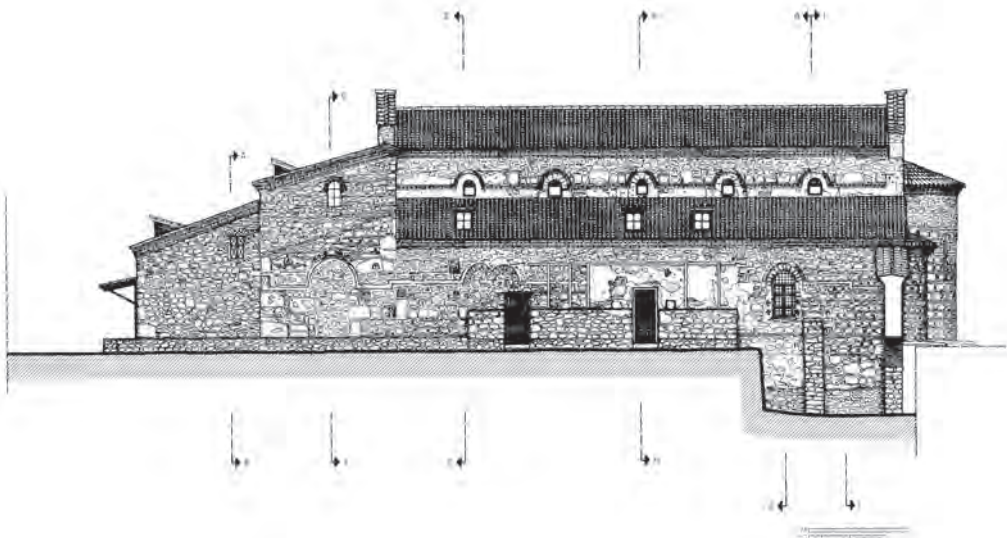
Fig. 8 Basilica of Dormition, Kalampaka, Thessaly, South elevation
