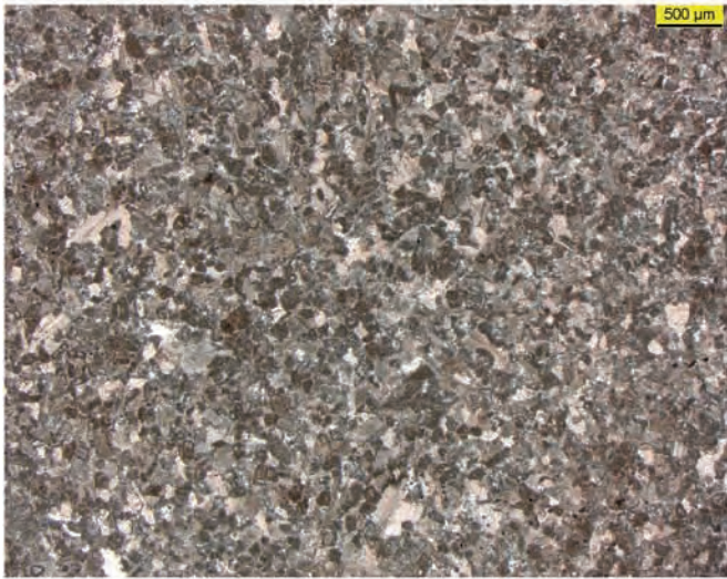
Abb. 12: Lithotyp F, Probe M15, DS//Pol
