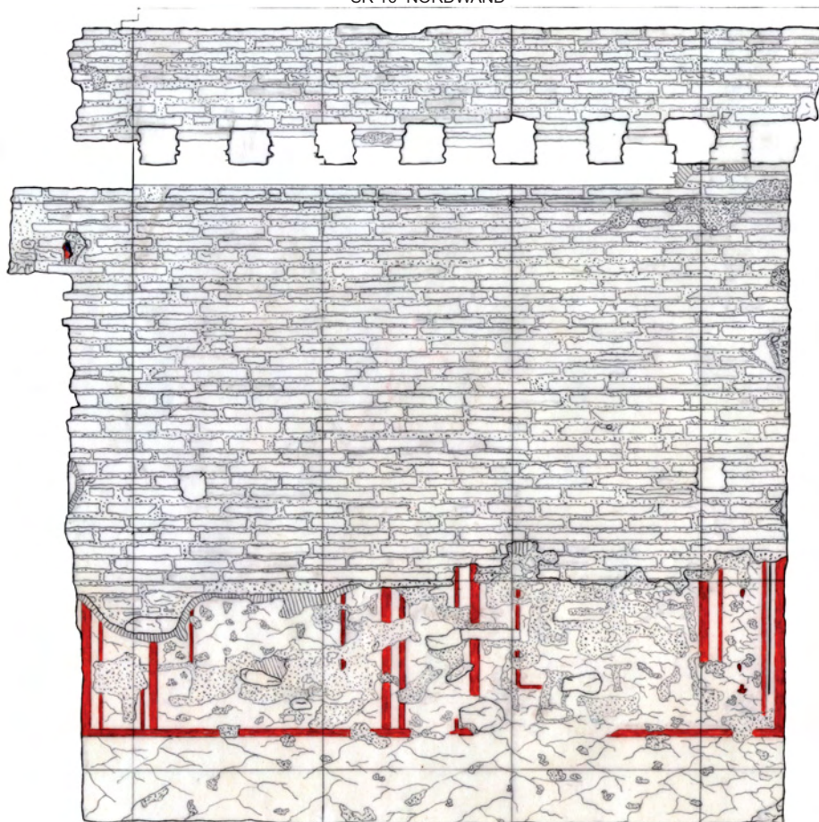
SR 16 OSTWAND
