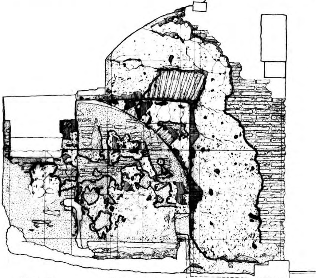
SR 2a WESTWAND
