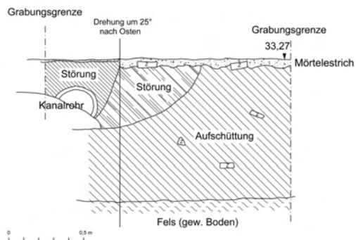
Abb. 8: SR 27, Sondage 5/97, O-Profil
