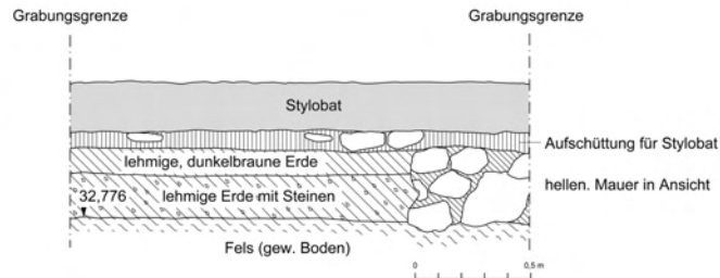
Abb. 7: SR 27, Sondage 5/97, W-Profil
