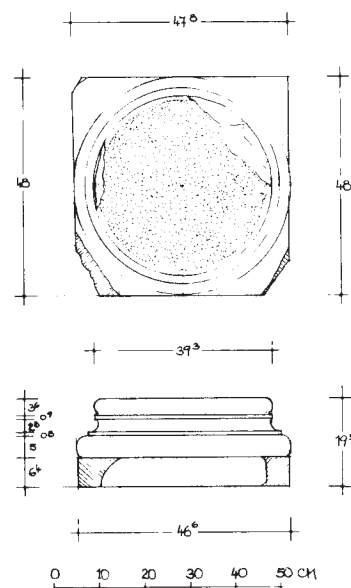
Abb. 58: Basis A55
