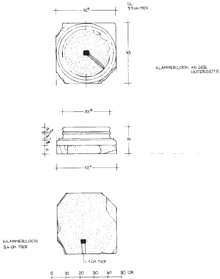
Abb. 108: Basis A88
