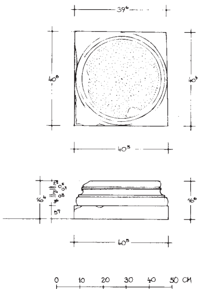
Abb. 50: Basis A51
