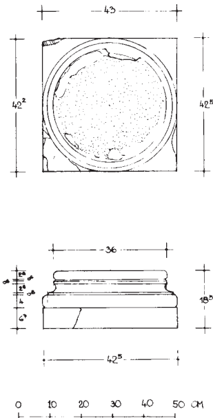
Abb. 52: Basis A52
