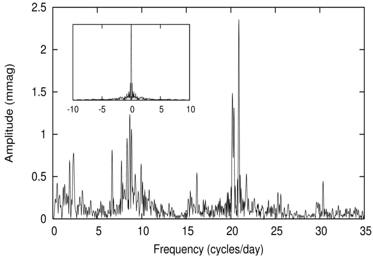
Figure 1: Fourier Spectrum of HD 114839, after removal of known instrumental artifacts. Inset is the window function for the highest peak in the spectrum.
