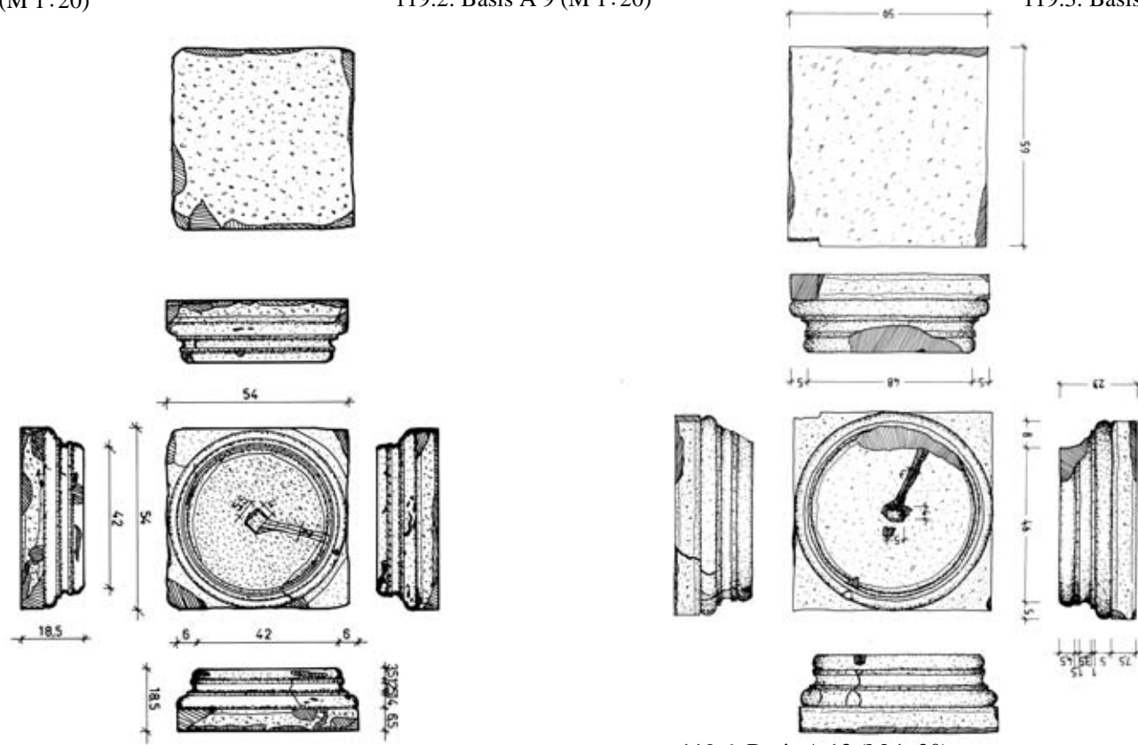
119.4: Basis A 11 (M 1:20)
