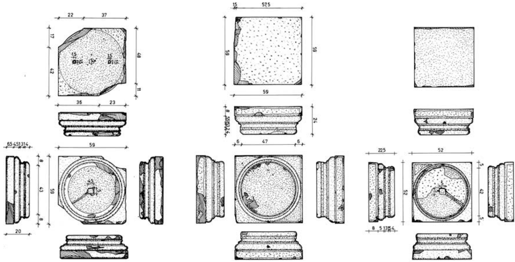
119.1: Basis A 1 (M 1:20)
