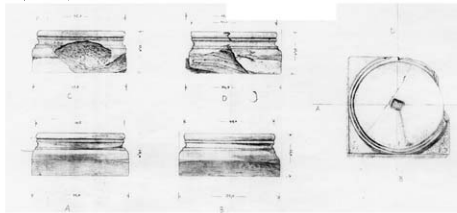
119.6: Basis A 13 (M 1:20)
