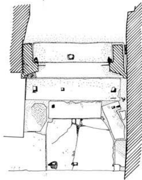
118.2: Grundriß prothyron (M 1:40)
